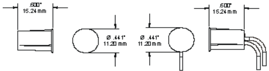
SWITCH
