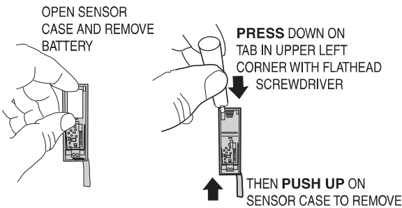
Figure 7. Removing Sensor from Wall/Mounting Plate
