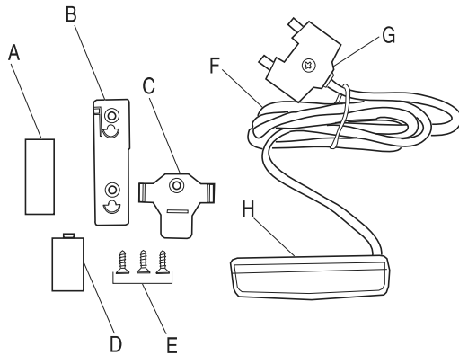
Figure 1. Temperature/Flood Sensor Contents
