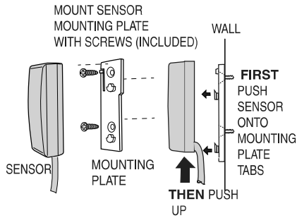
Figure 6. Screw Mounting Sensor Mounting Plate
