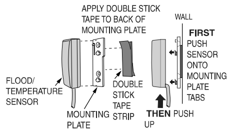
Figure 5. Double Stick Tape Mounting Sensor Mounting Plate
