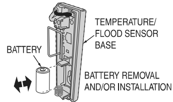
Figure 4. Installing New Battery
