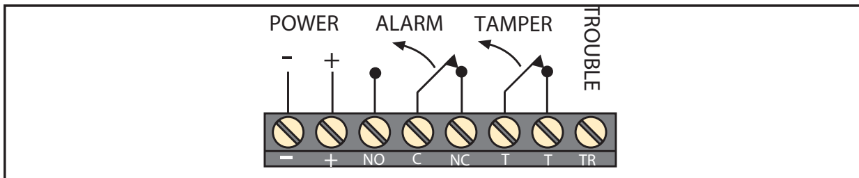
Figure 3.1: Wiring to terminals
