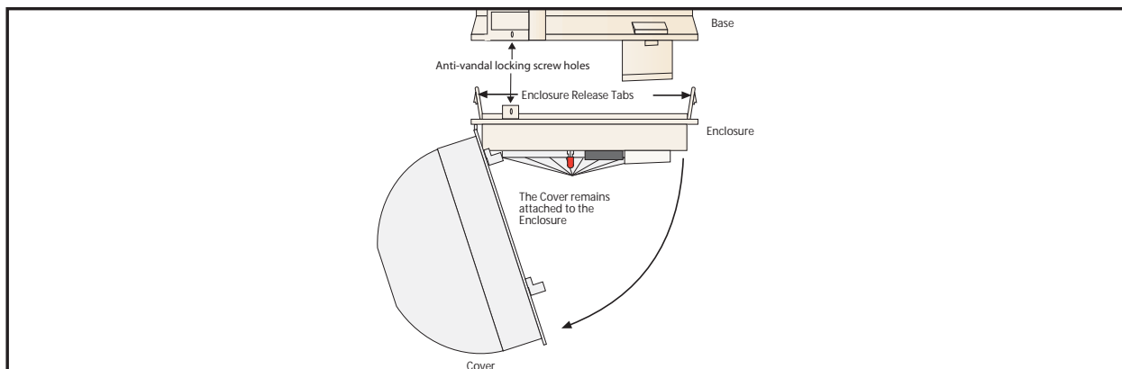
Figure 2.1: Opening cover
