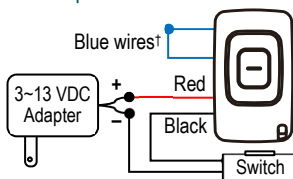
Fig. 2 External inline power-on switch
