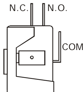
TERMINAL TYPE: .250" QUICK CONNECT
